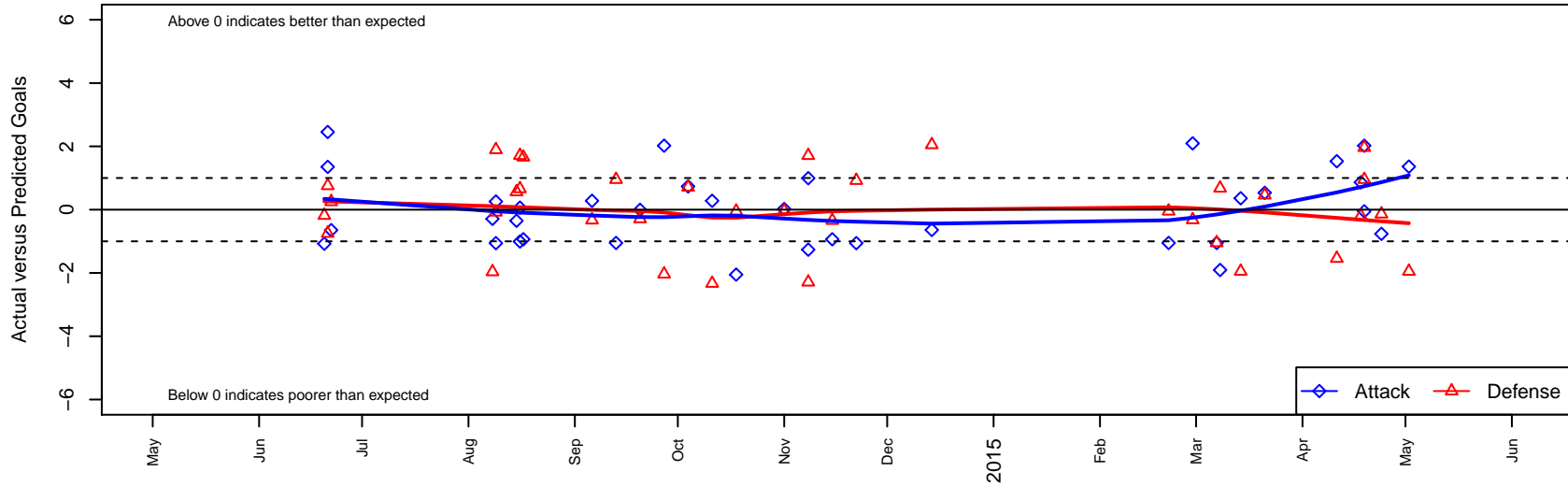
NW United Premier G01 Dots are actual minus expected GF (blue circles) and GA (red triangles). Blue line is smoothed change in attack strength. Red is smoothed change in defense strength.
